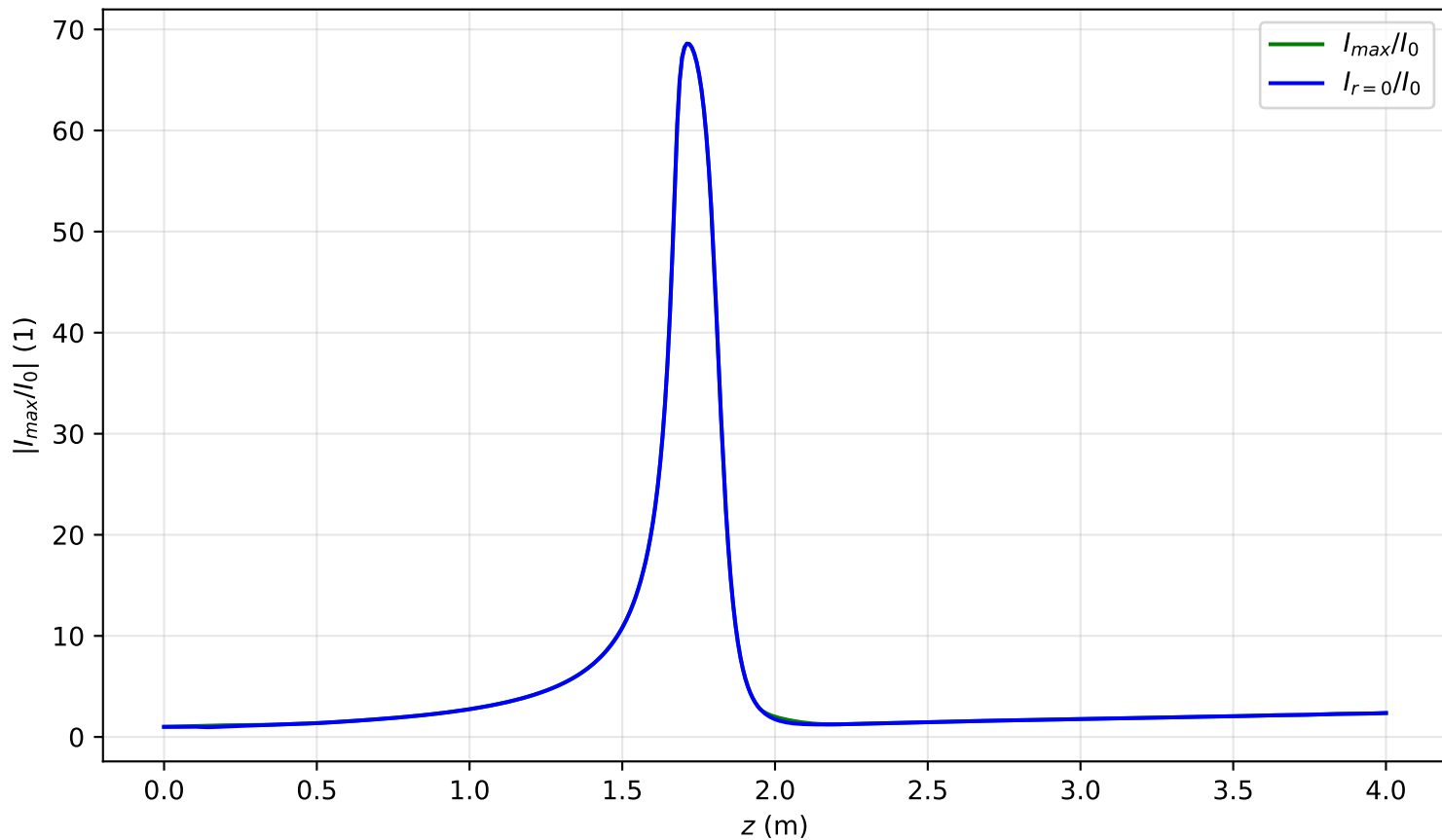
I_{max}(x=0, y=0, z)/I_0 , Pin=1.5Pcr, noisy input, artificial time
